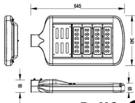
Outline Dimensions
