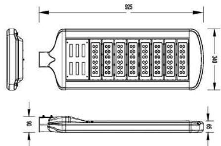
Outline Dimensions
